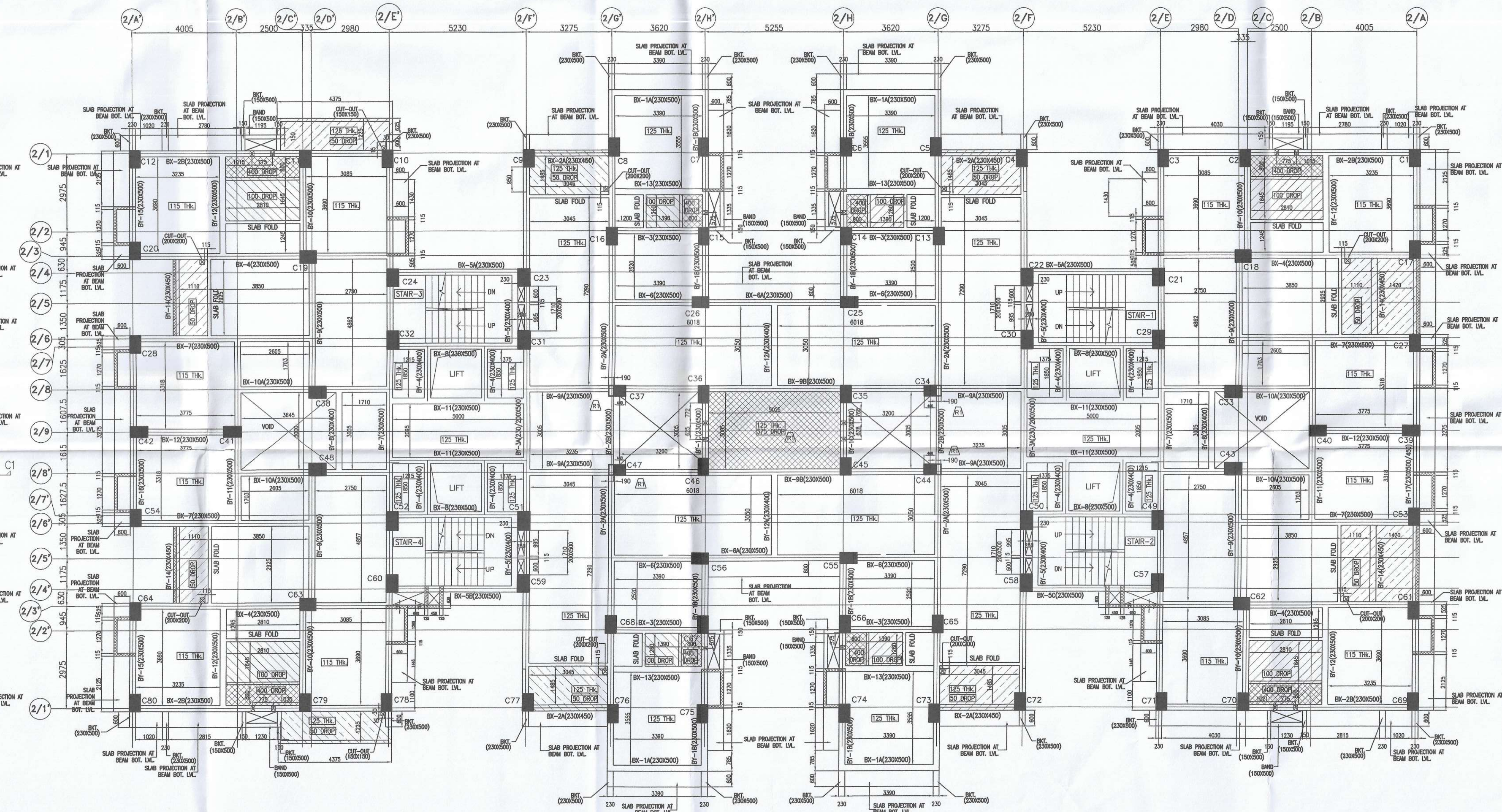
G.A. OF 10TH FLOOR (BLOCK-2) ALL SLAB THICKNESS 100mm EXCEPT NOTED
